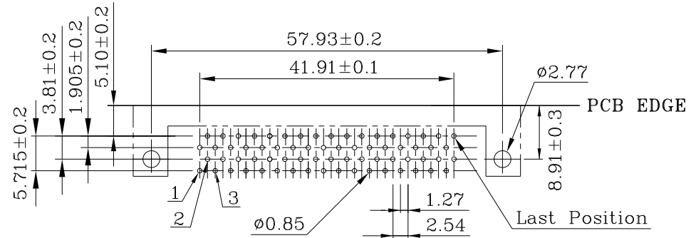
PCB Layout
