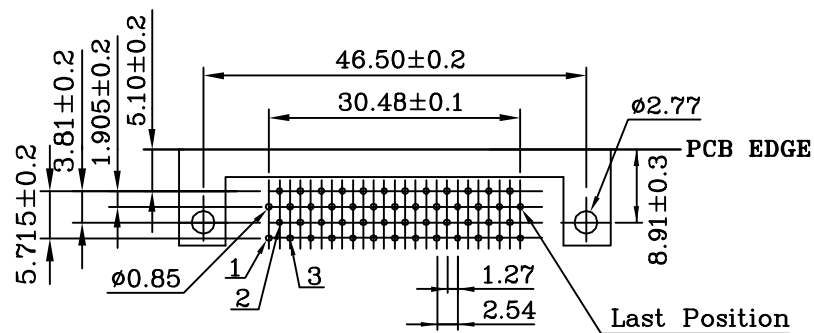
PCB Layout
