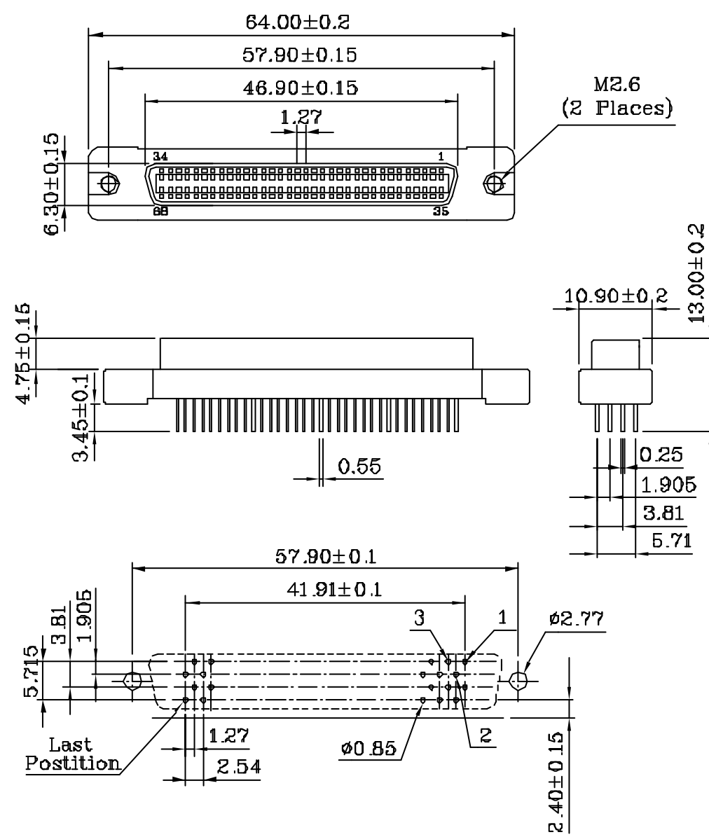
PC Board Mounting Dimensions
