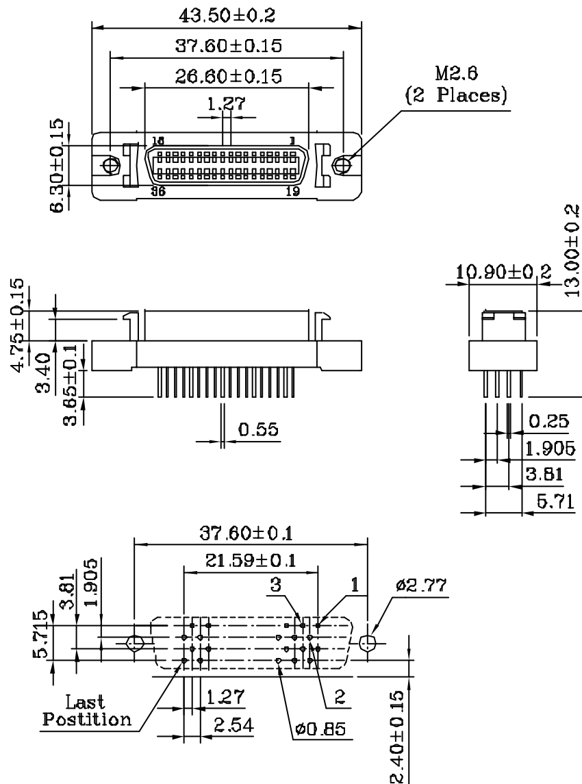
PC Board Mounting Dimensions
