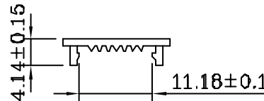
Termination Cover (1 Places)
