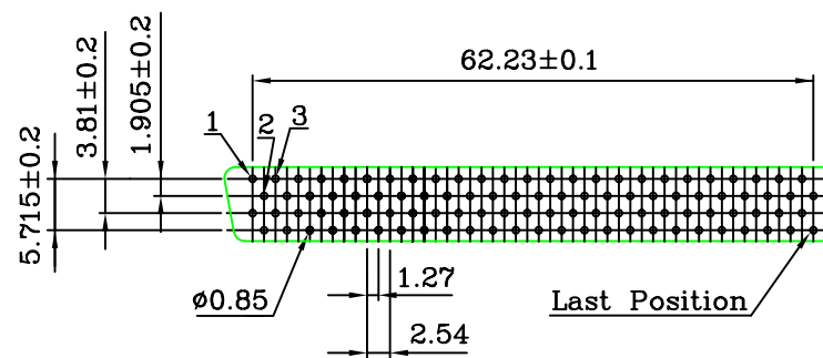
PCB Layout
