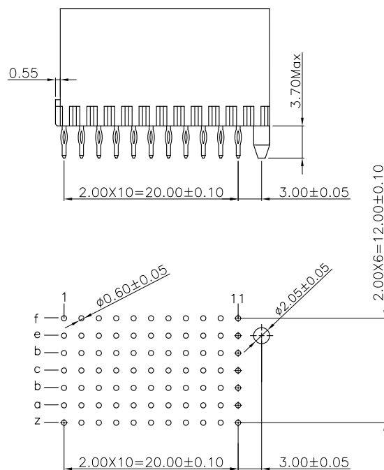
P.C. Board Layout (Top View)
