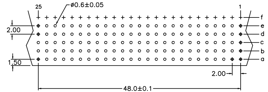
P.C. Board Layout (Top View)
