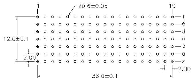
P.C. Board Layout (Top View)
