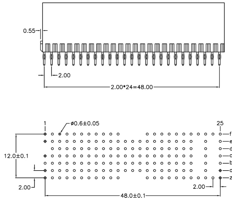
P.C. Board Layout (Top View)
