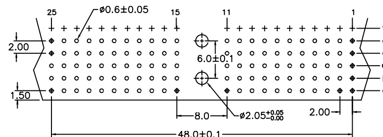
P.C. Board Layout (Top View)
