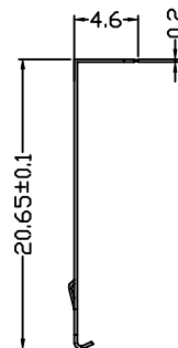
Bottom Shielded
