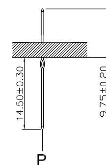
Contact Layout
