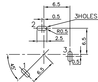
T:1.6 Dimensions of PC board holes Tolerance : \pm 0.05 (Printed-top view)
