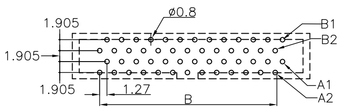
P.C. Board Layout Top View (Tolerance: ±0.05) (20,32,40,52,60,68,80,100 Position)
