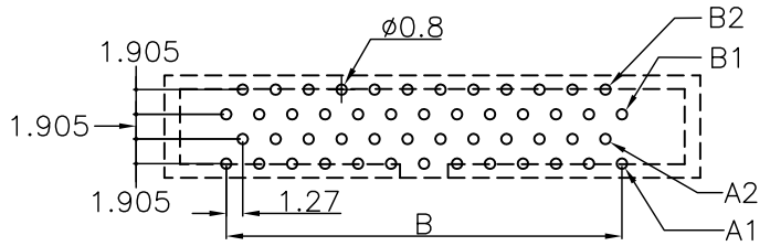
P.C. Board Layout Top View (Tolerance: ±0.05) (26,34,50 Position)
