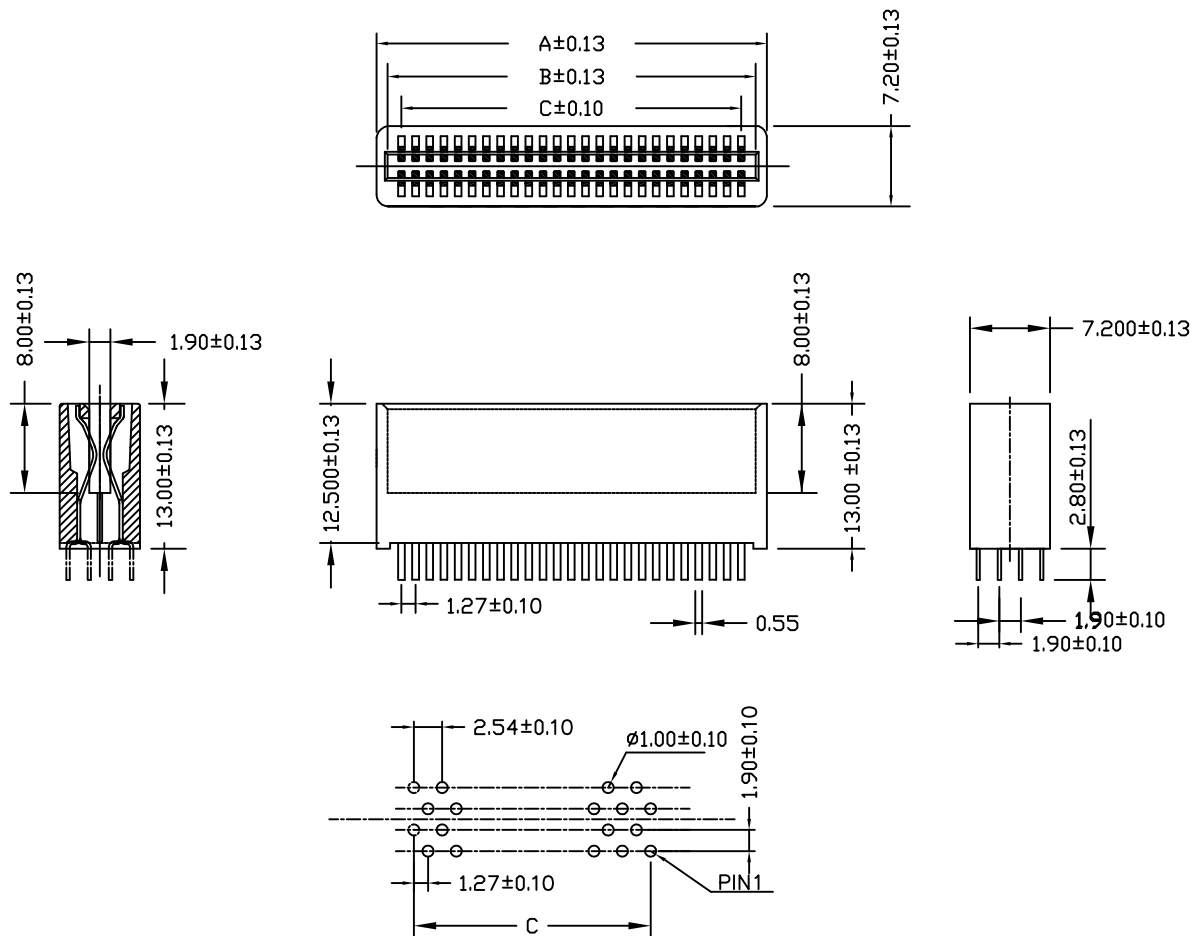
RECOMMENDED PCB LAYOUT FOR EVEN NUMBERS (TOP VIEW)
