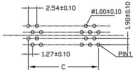
RECOMMENDED PCB LAYOUT FOR EVEN NUMBERS (TOP VIEW)
