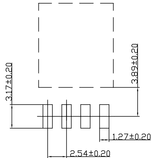
P. C. B Hole Layout
