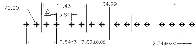
PCB Layout
