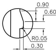
View "C"
