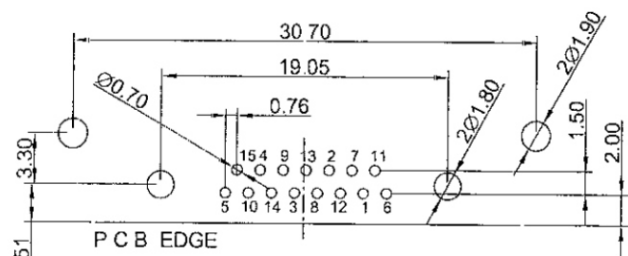
RECOMMENDED P.C.B HOLE LAYOUT COMPONENT SIDE VIEW(TOLERANCE ±0.05mm)
