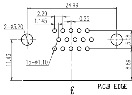
RECOMMENDED P.C.B LAYOUT INSPECTION DIMENSION:(A)~(H)
