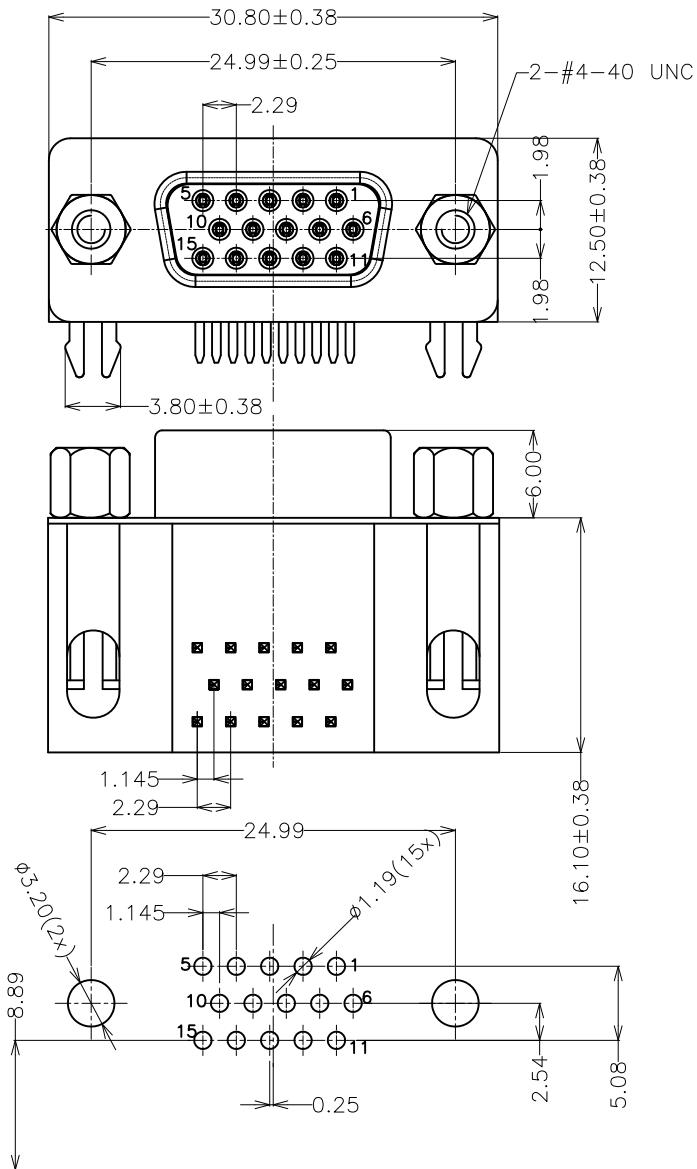
P.C.B. LAYOUT TOP VIEW
