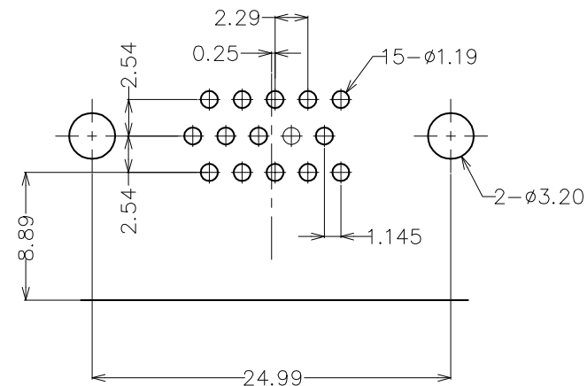
P.C.B. LAYOUT (TOLERANCE \pm 0.05 ) TOP VIEW
