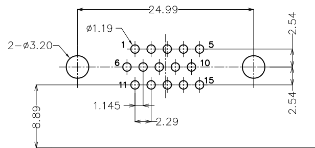
P.C.B. LAYOUT(TOLERANCE±0.05) TOP VIEW
