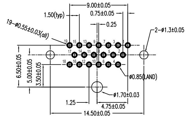
RECOMMENDED PCB LAYOUT(t=1.20±0.15)
