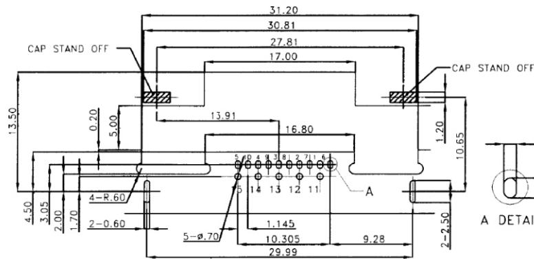
RECOMMENDED P.C.B LAYOUT (COMPONENT SIDE) THICKNESS:1.2mm GENERAL TOLERANCE:±0.05mm
