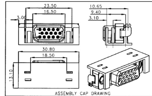
ASSEMBLY CAP DRAWING
