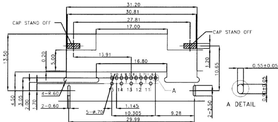
RECOMMENDED P.C.B LAYOUT (COMPONENT SIDE) THICKNESS:1.2mm GENERAL TOLERANCE:±0.05mm
