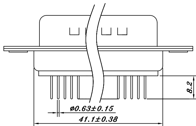
44PIN MALE MACHINED PIN
