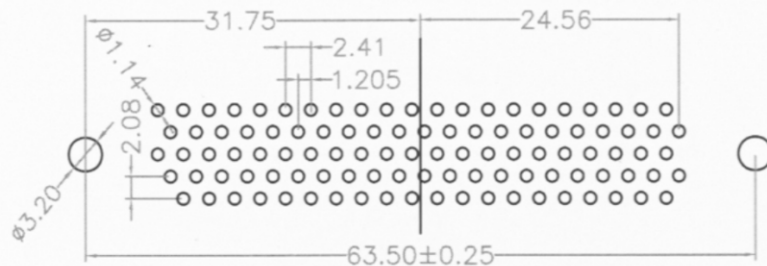
Recommended mounting hole pattern for 3.4mm thick P.C Board
