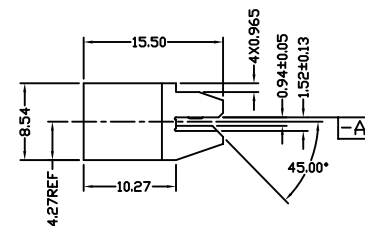
VIEW C-C
