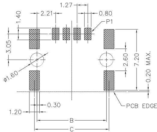
P.C.Board Layout TOLERANCE: ±0.05
