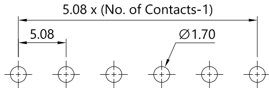
Recommended PCB Layout (PCB Board Tolerance±0.05)
