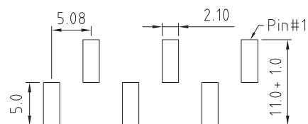
RECOMMENDED PCB SMT LAYOUT (TOLERANCE: ±0.05mm)
