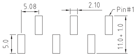
RECOMMENDED PCB SMT LAYOUT (TOLERANCE: ±0.05mm)
