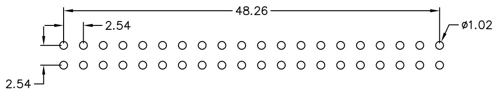
Recommended P.C.B Layout
