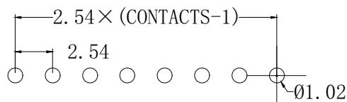
P. C. B . LAYOUT
