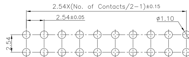
PCB Layout
