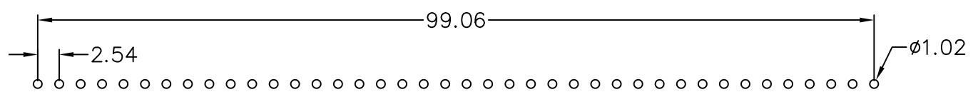
Recommended P.C.B Layout
