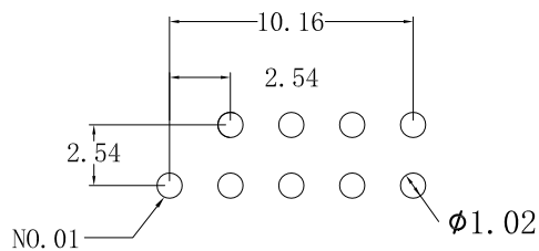
P. C. B . LAYOUT
