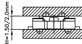
MATED DRAWING (REF) SCALE : 5 : 1
