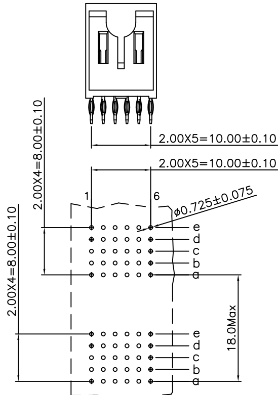
P.C. Board Layout (Tolerance: \pm 0.05 )
