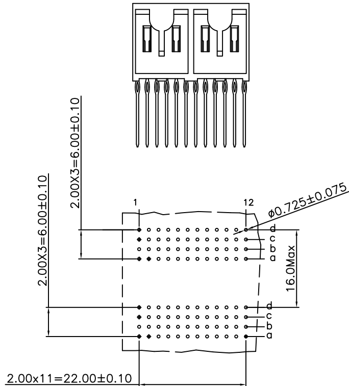
P.C. Board Layout
