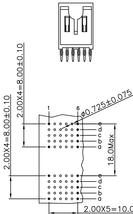
PCB Layout
