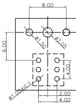
P.C. Board Layout Tolerance±0.05
