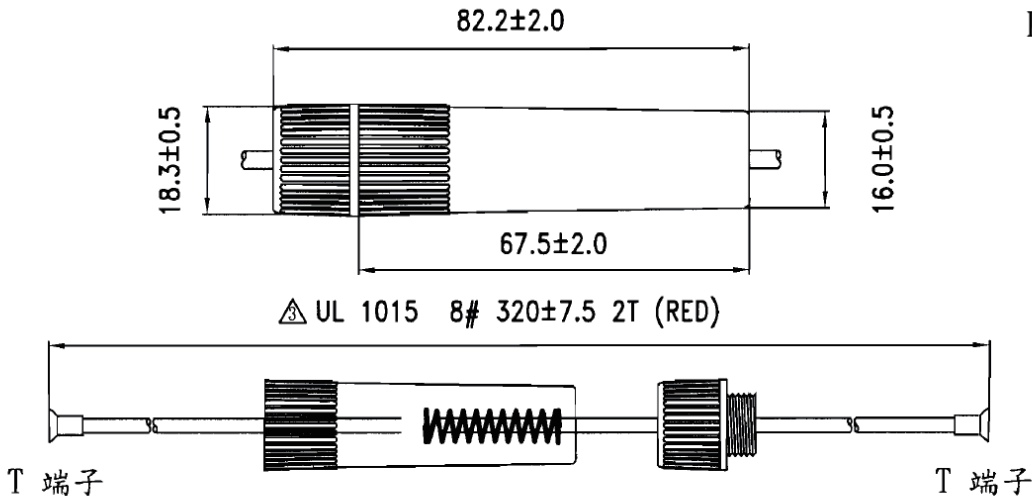
IN-LINE FUSE HOLDER AUE (10.3 x 38.1mm) FUSES
