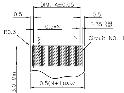
RECOMMENDED APPLICABLE FPC LAYOUT (THICKNESS: 0.3±0.03)
