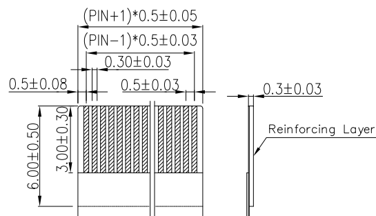
RECOMMENDED FFC TOLERANCE: ±0.05
