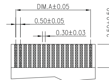
FFC/FPC DIMENSION THICKNESS 0.30 \pm 0.03\text{mm}
