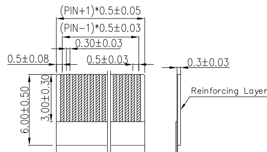
RECOMMENDED FFC TOLERANCE: \pm 0.05
