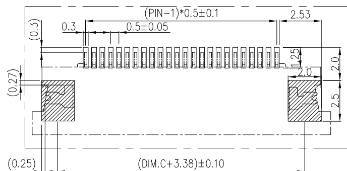
RECOMMENDED PCB LAYOUT TOLERANCE: \pm 0.05
