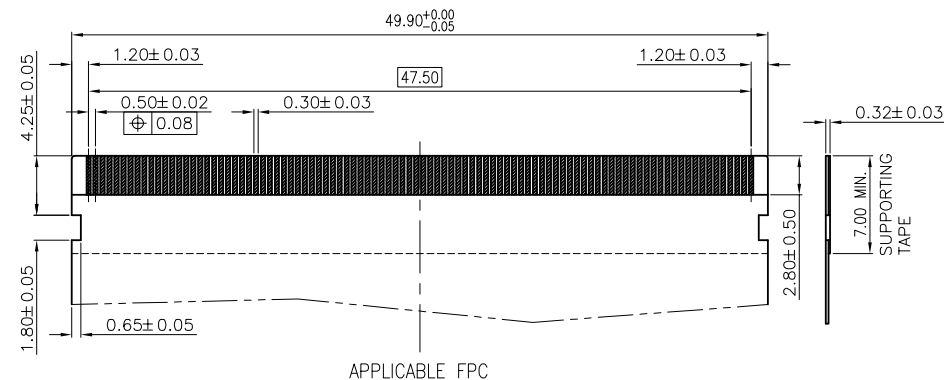
APPLICABLE FPC
